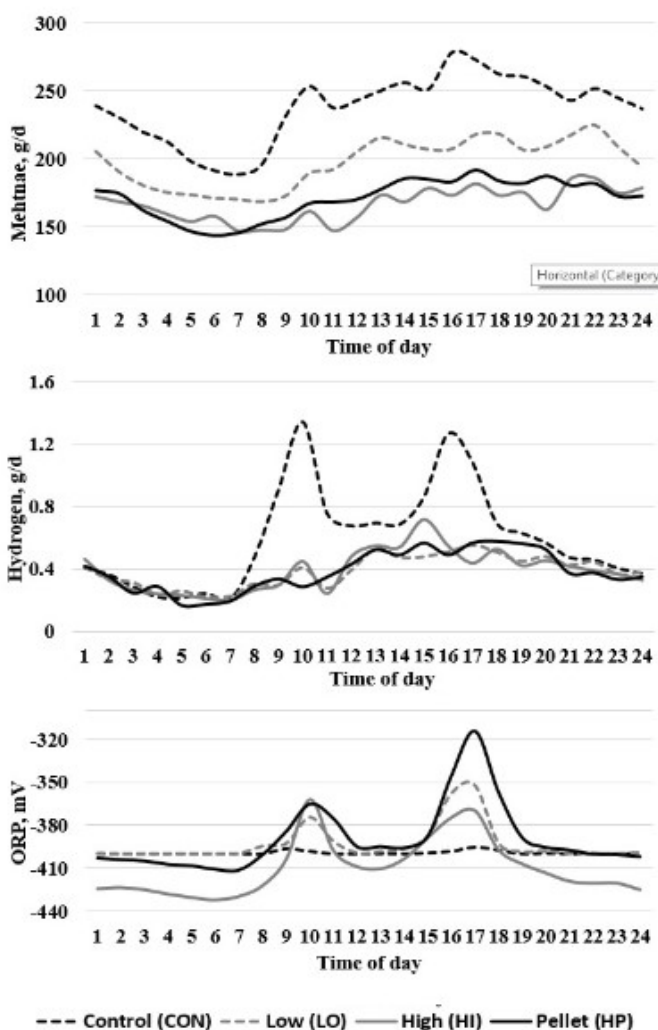
FIGURE 1. ASSESSING \text{CaO}_2 IN A TWICE DAILY FEEDING REGIMEN (0800 H, 1500 H) IN BEEF CATTLE. DIURNAL PATTERN OF DAILY \text{CH}_4 (G/D), \text{H}_2 (G/D) AND ORP (MV). SOURCED FROM ROSKAM ET AL. (2023A).
